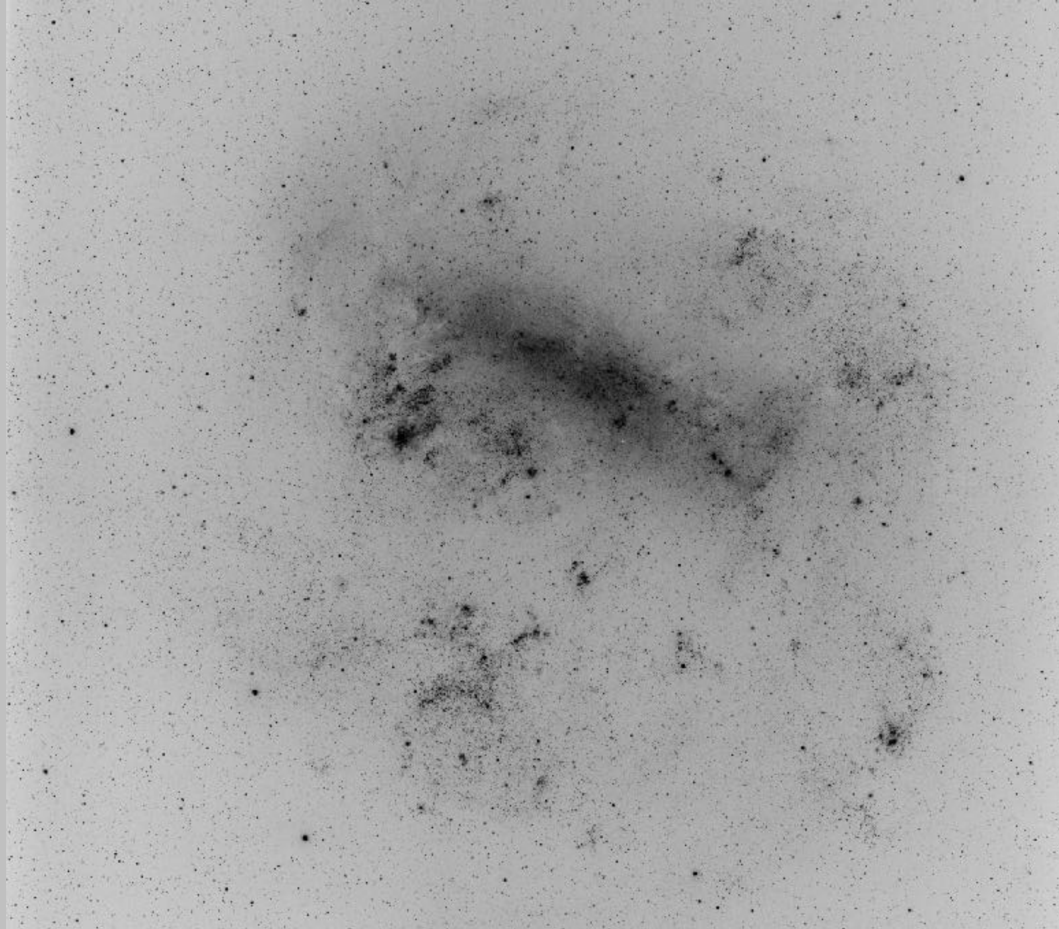
Photographic plate showing the Large Magellanic Cloud (Boyden Observatory, 1966) | Rüdiger Knigge
