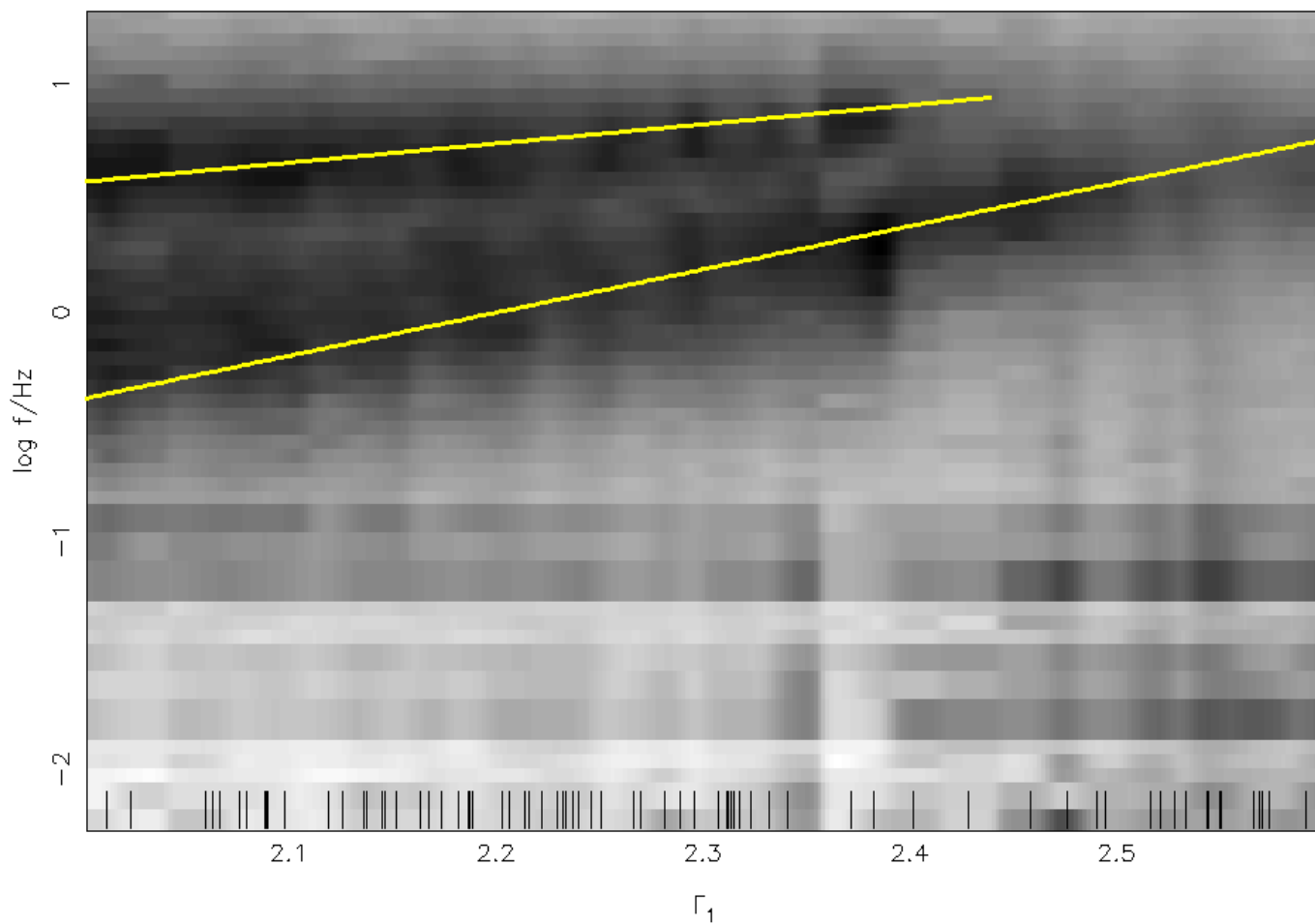
PSDs of Cygnus X-1 in the higher energy band
