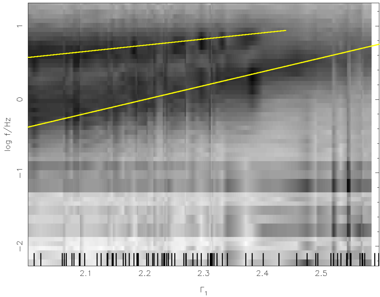
PSDs of Cygnus X-1 in the lower energy band
