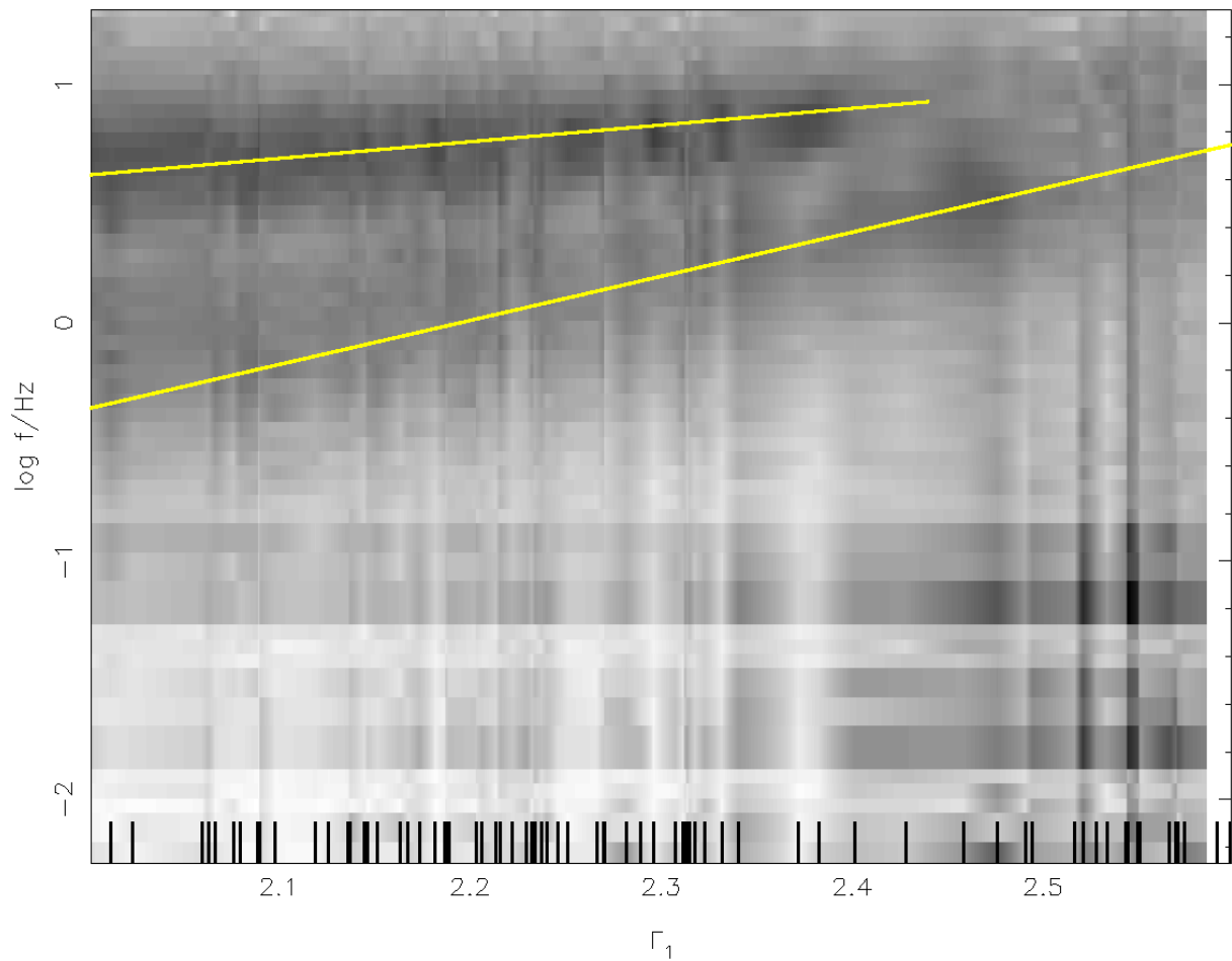
PSDs of Cygnus X-1 in the higher energy band
