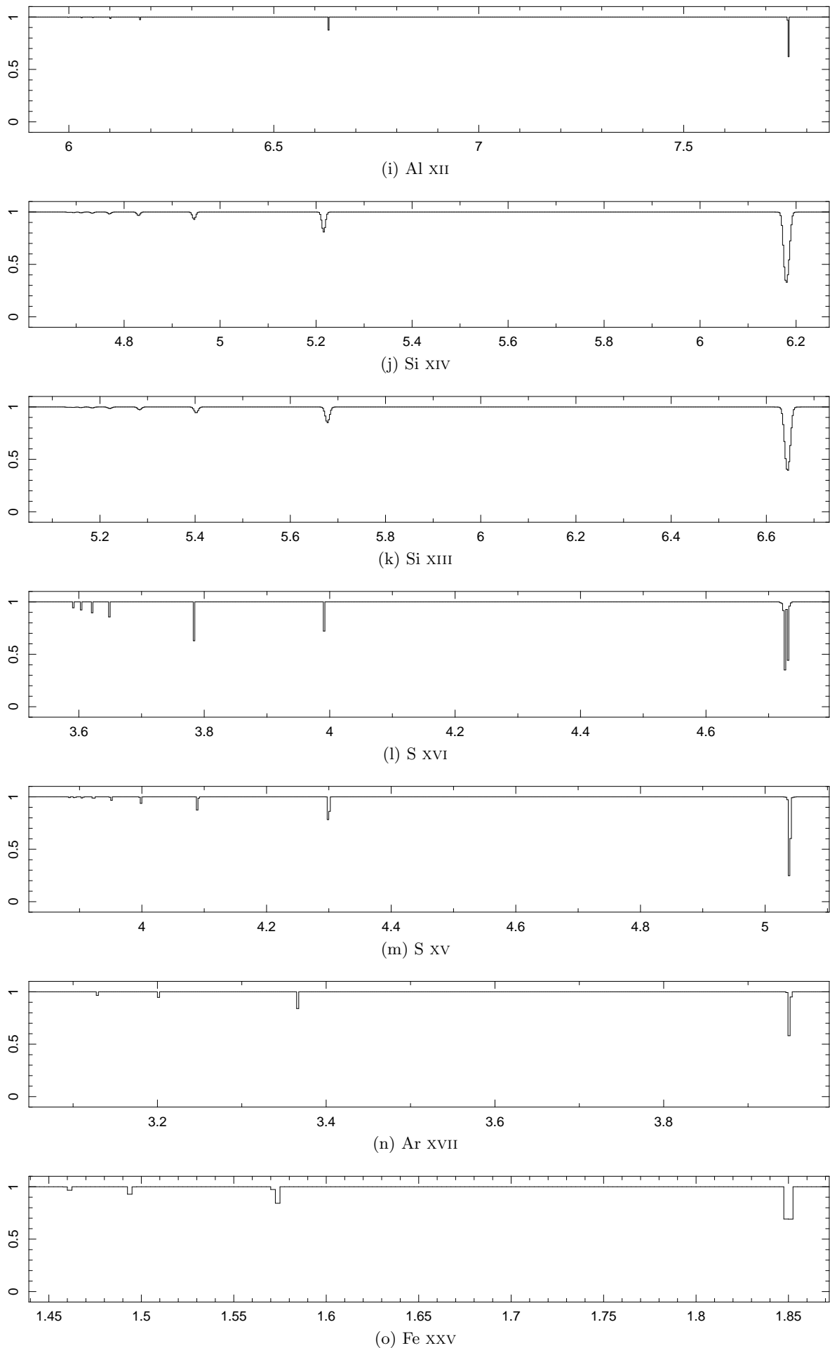
Fig. 4.14: Line profiles of the fitted series vs. wavelength in Å (continued on next page).
