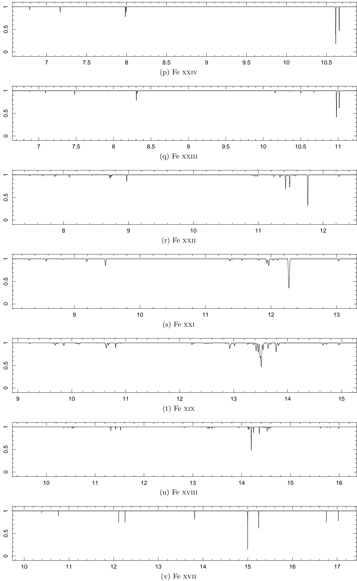
Figure 4.1: Line profiles of the fitted series vs. wavelength in \text{\AA} .
