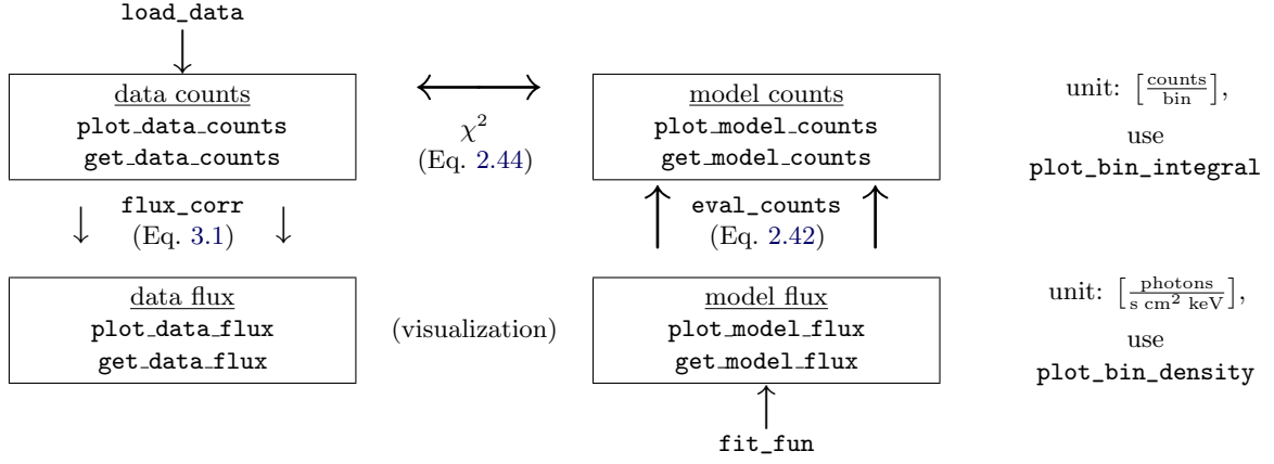
Figure 3.1: The main data structures for spectral analysis in ISIS and their interactions.
